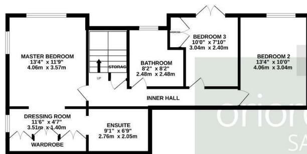
GROUND FLOOR 692 sq.ft. (64.2 sq.m.) approx.
