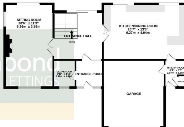
1ST FLOOR 973 sq.ft. (90.4 sq.m.) approx.
